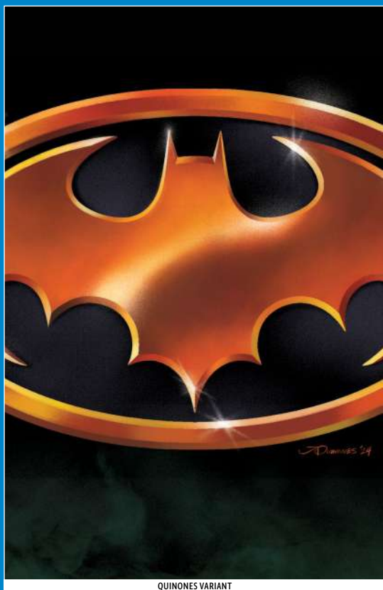
QUINONES VARIANT
